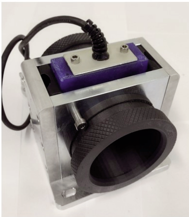
Figure 4 - CP65-NS with fixed center coil and built-in bushings
