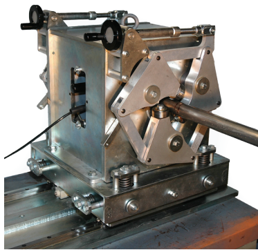
Figure 9 - 65mm Coil Platform for encircling or segmented eddy current applications, uses an electro magnet to saturate the material.
