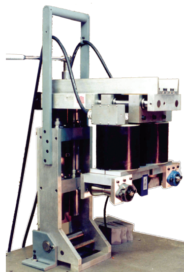
Figure 7 - CP 850 Coil Platform uses a tangent coil, and large electromagnets, shown above, for saturation. The unit tilts back to allow convenient changes in the coil for different material sizes.
