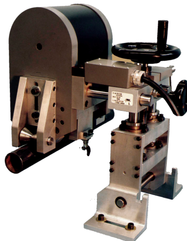
Figure 8 - CP 354 Tangent Coil Platform for Testing Magnetic Material
