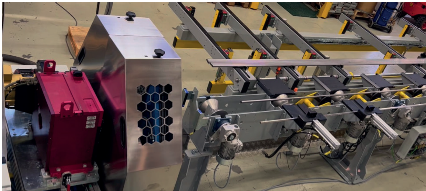
Figure 2: Eddy Current Rotomac® rotary tester, at left, with automated feed system at right, part of a 32M long system for inspecting cold finished, close tolerance round bar. The system also includes an Echomac® ultrasonic rotary tester.
